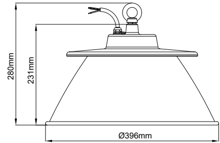
Tall Reflector
