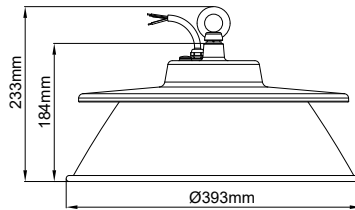
Universal Reflector
