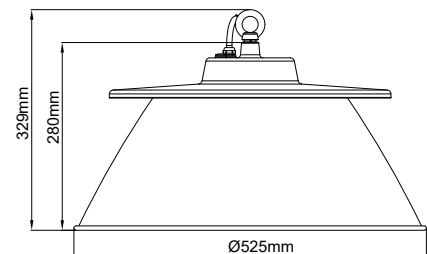
Tall Reflector
