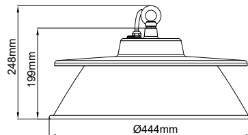
Universal Reflector
