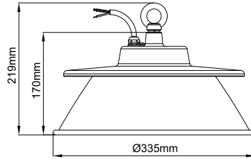
Universal Reflector
